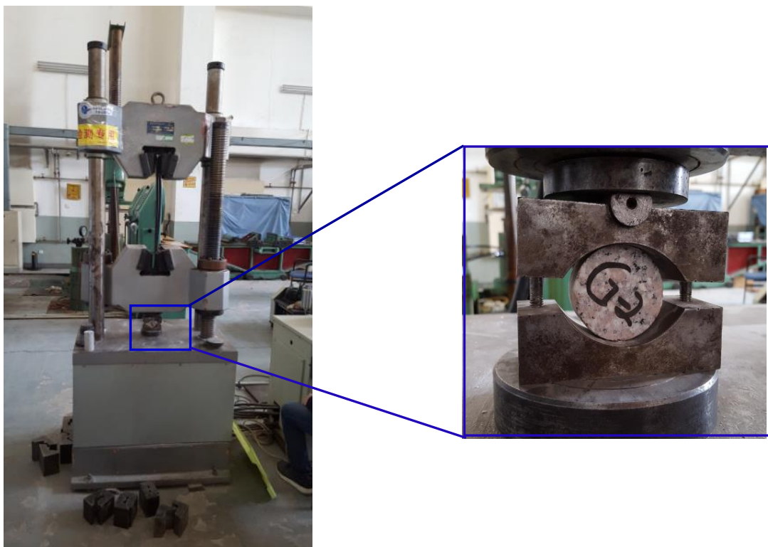
Fig.2 - Hydraulic testing machine for Brazilian test
