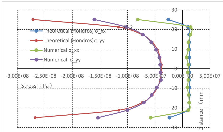
Fig.9 - Theoretical and numerical results of stresses distribution across loaded diameter for disc specimen
