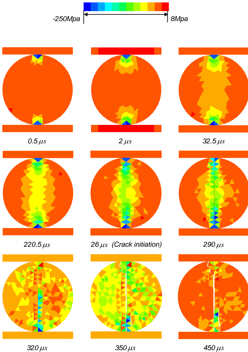
Fig.5 - Stress propagation process of BTS test
