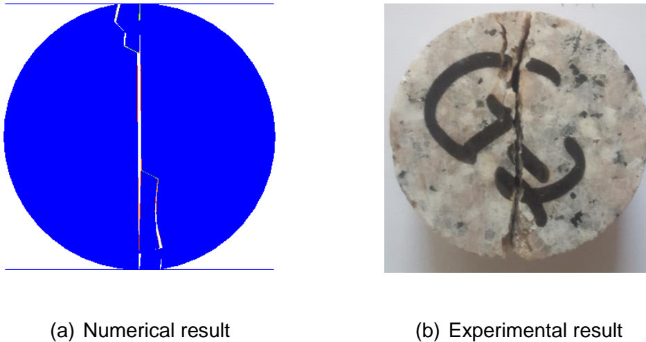
Fig.7 - Comparison of the numerical and experiential results
