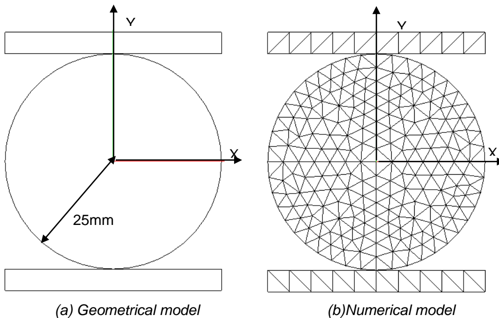
Fig.4 - Geometrical and Numerical model for BTS test
