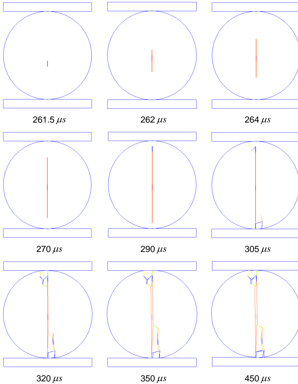
Fig.6 - Crack initiation and propagation of BTS test
