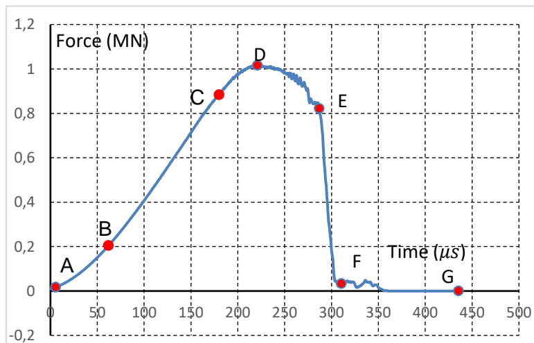
Fig.8 - Force-loading displacement curve
